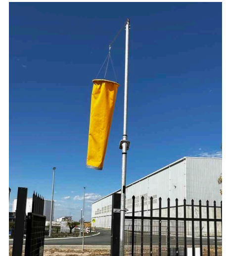
Mid and base hinging poles, providing safe and cost effective solutions - eliminating the need for elevated work platforms
