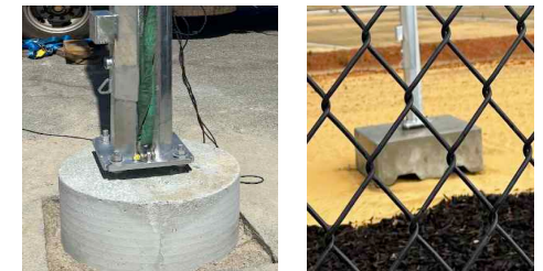
A variety of Pile Type or Pre-Cast Concrete footings are available. The pole can also be Chemically Anchored to a suitable pad
