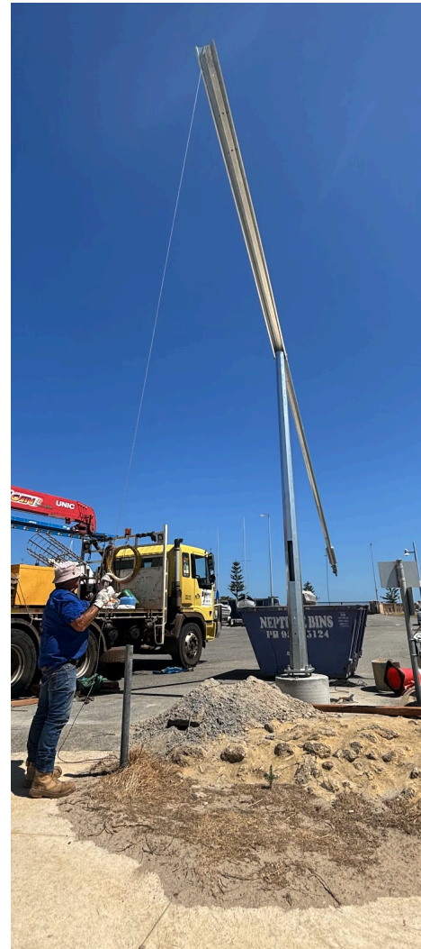
The design of the mid hinging, counterweighted pole eliminates the need for an elevated work platform, with all work able to be carried out at ground level
