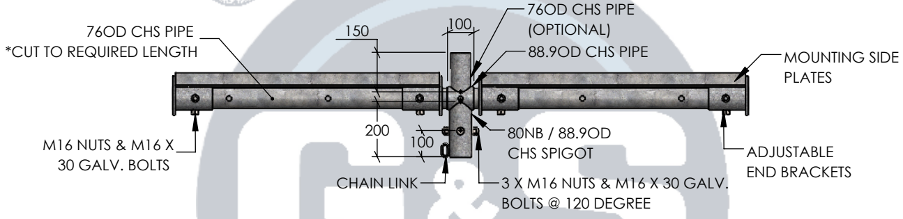
FRONT VIEW SCALE 1:20
