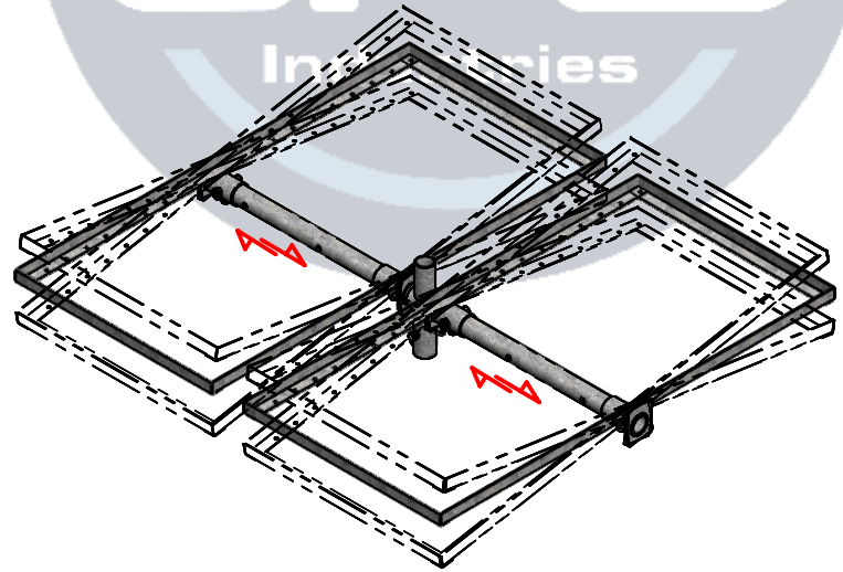
ISOMETRIC VIEW SCALE 1:30
