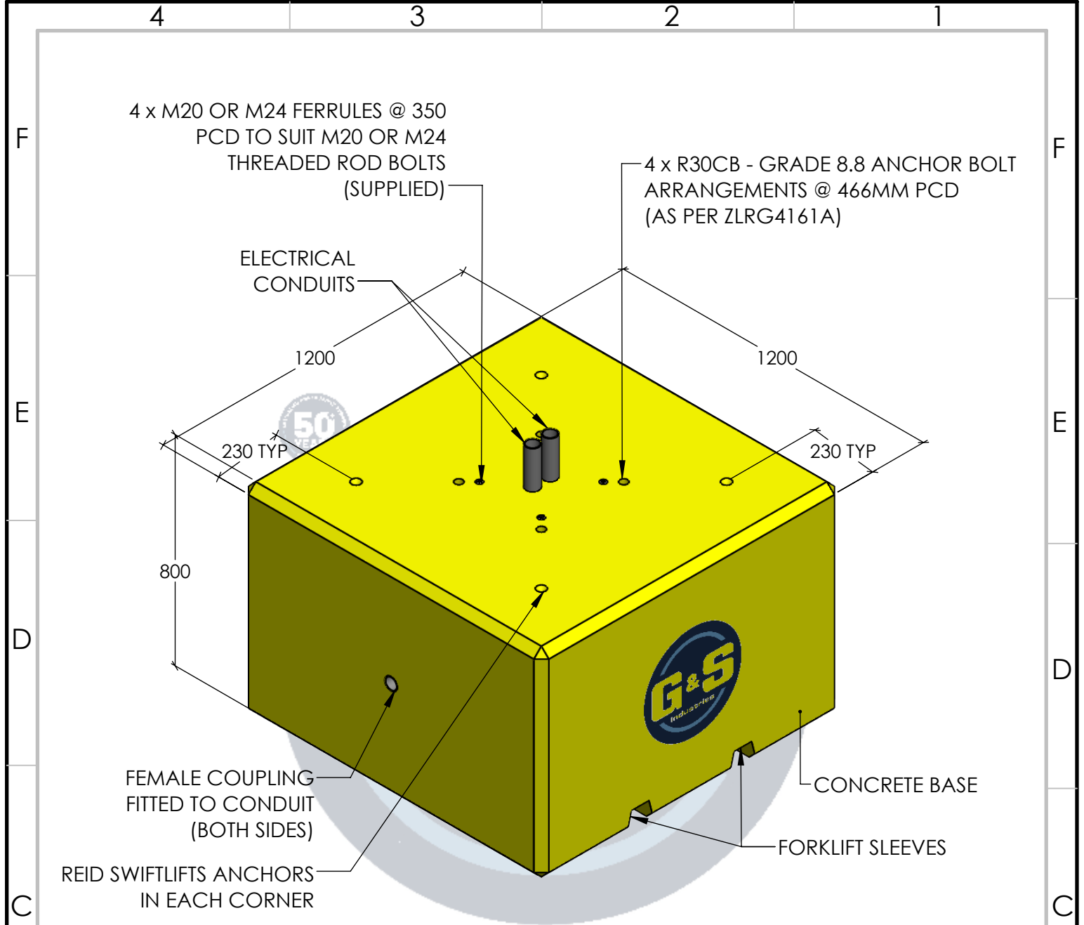
3D VIEW SCALE 1:20
