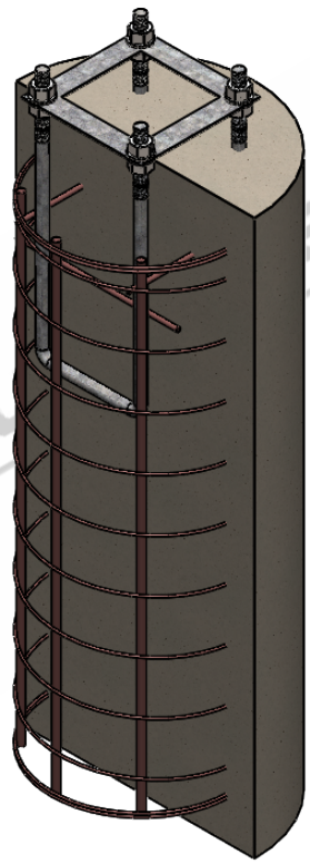
ISOMETRIC VIEW SCALE 1:15
