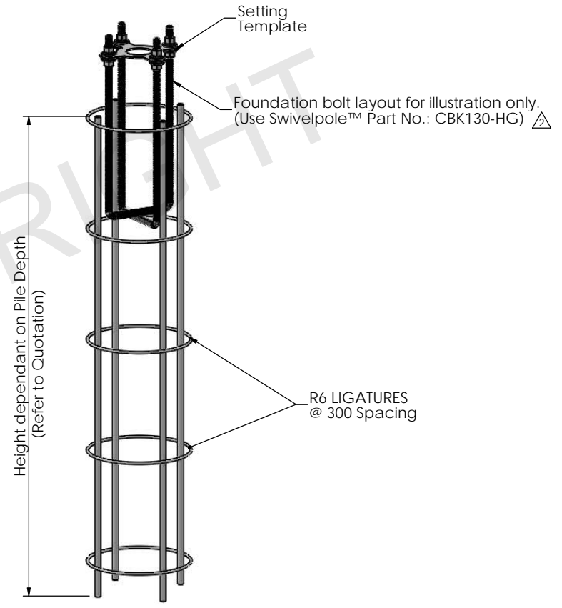
F7-M2 & G5 TYPICAL ASSEMBLY (Reinforcement Cage)
